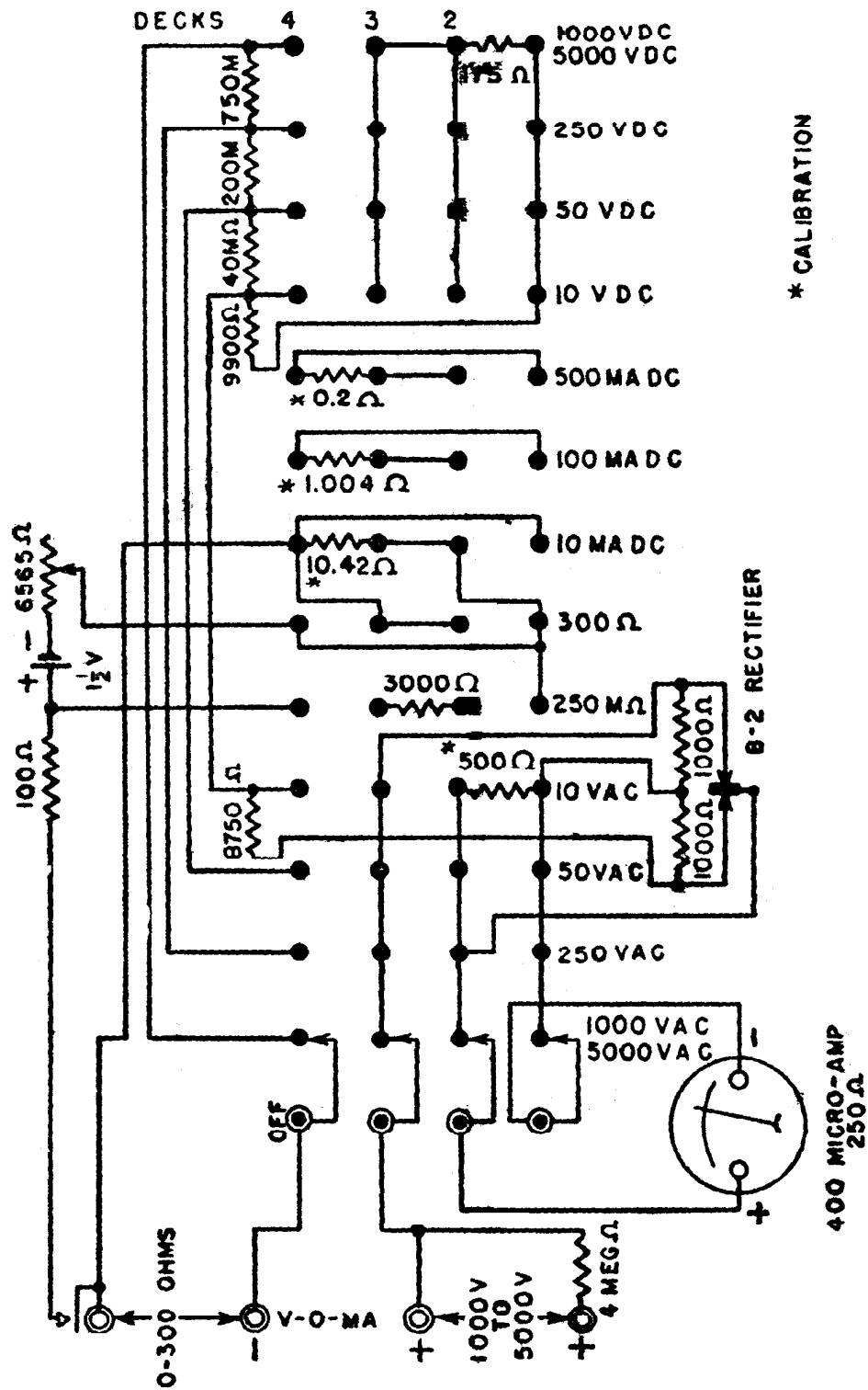
MODEL 666-H WIRING DIAGRAM
